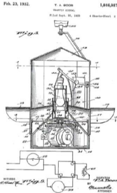
This is an internal schematic of the electric system for the original signal that hung at the corner of Long and Main Streets.
