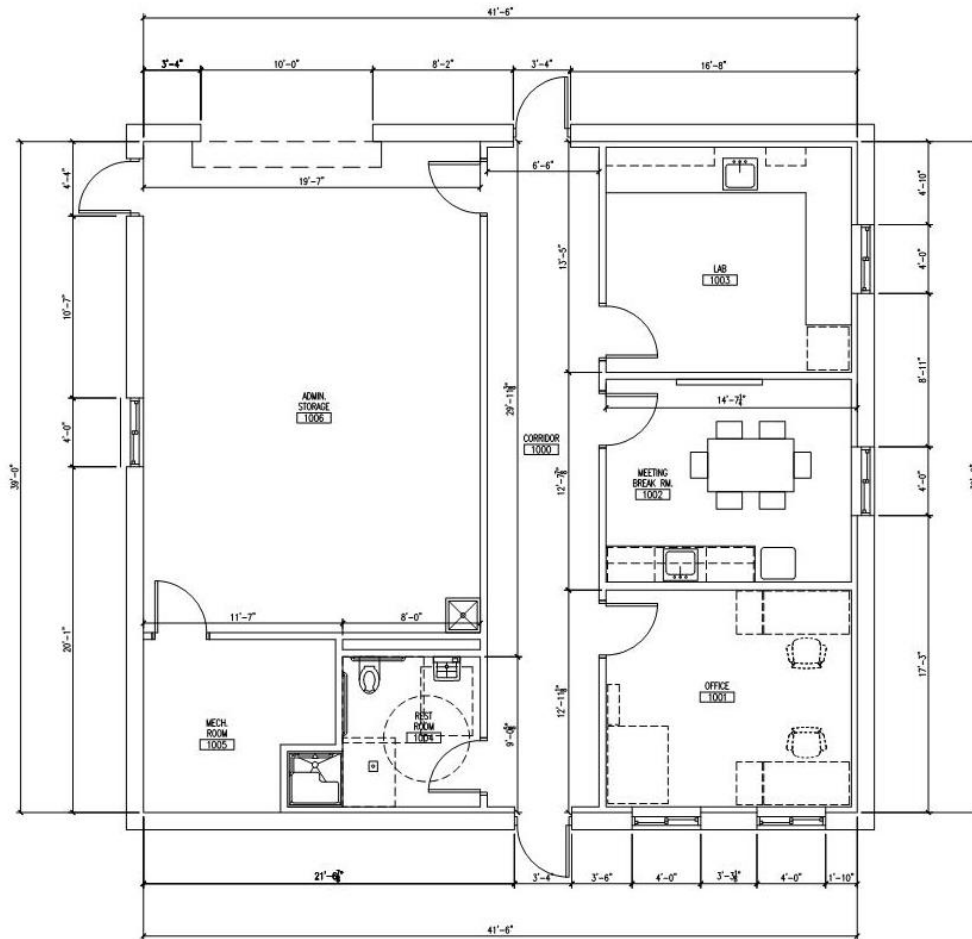
1 FLOOR PLAN SCALE: 1/4" = 1'-0"
